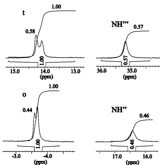
Figure 7. The fragments of the 1 H NMR spectrum (298 K, CD 3 OD/CDCl 3 1:2 v/v) of the partially deuterated ( M )-[EuL RRRRRR ](NO 3 ) 3 ·4H 2 O complex illustrating the doubling of the signals o and t , correlated to the changes of intensity of signals NH'' and NH''' , respectively.
