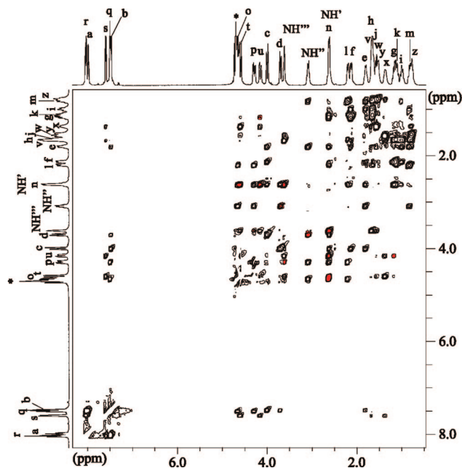
Figure 5. The ROESY spectrum of the (P) -[LuL R RRRRR](NO 3 ) 3 ·7H 2 O complex ( D_2O , 298 K). Red color indicates the cross-peaks corresponding to short distances characteristic for the twisted form of the macrocycle (see text for details).
