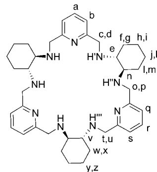
Scheme 1. Macrocycle L RRRRRR and Its Labeling
