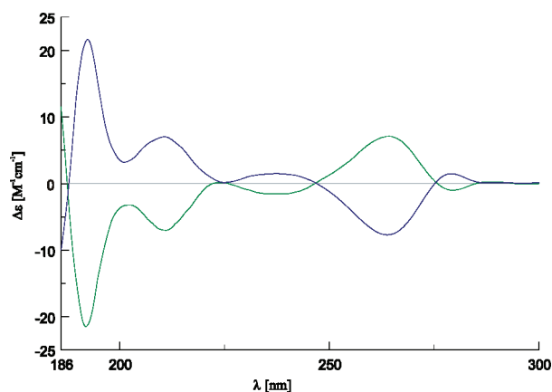
Figure 2. CD spectra of the two enantiomeric [\text{NdL}](\text{NO}_3)_3 \cdot 0.5\text{H}_2\text{O} complexes in 1 \times 10^{-3} M \text{H}_2\text{O} solutions: (M) - [\text{NdL}_{\text{RRRRRR}}]^{3+} (green) and (P) - [\text{NdL}_{\text{SSSSSS}}]^{3+} (blue).
