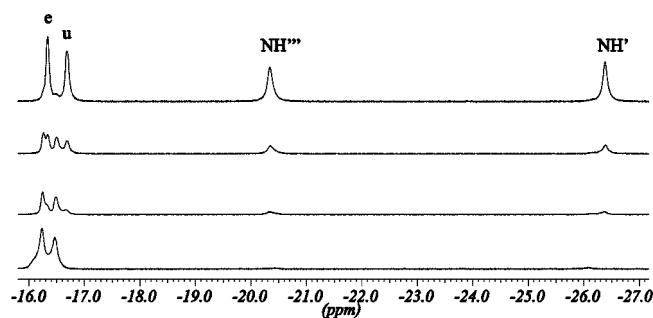
Figure 8. The fragments of the 1 H NMR spectra recorded over 27 h (298 K, CD 3 OD/CD 3 CN) of the ( M )-[PrL RRRRRR ](NO 3 ) 3 ·H 2 O complex, illustrating the doubling of the resonances due to isotope effect. Spectra measured after (from top) 15 min, 2 h 30 min, 5 and 27 h.
