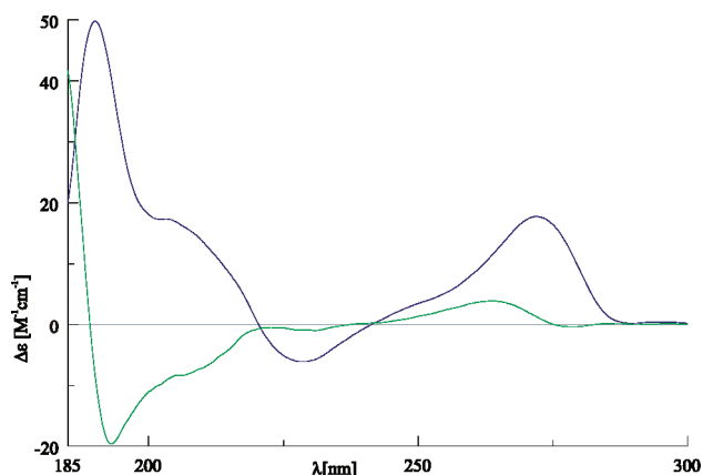
Figure 3. CD spectra of the two diastereomers of the Er(III) complexes with \text{L}_{\text{RRRRRR}} in 1 \times 10^{-3} M \text{H}_2\text{O} solutions: (M) - [\text{ErL}_{\text{RRRRRR}}]^{3+} (green) and (P) - [\text{ErL}_{\text{RRRRRR}}]^{3+} (blue).
