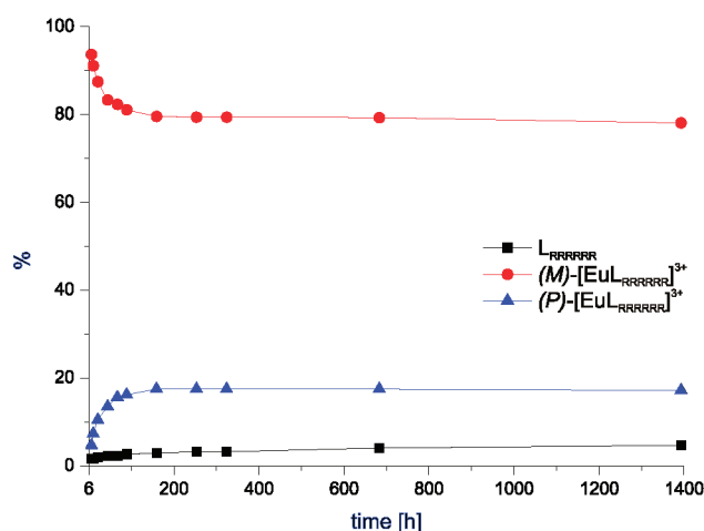
Figure 4. Dependence of the relative concentration of the (M) - and (P) -diastereomers on the heating time of 1 \times 10^{-2} M solutions of (M) - [\text{LnL}_{\text{RRRRRR}}](\text{NO}_3)_3 complexes ( \text{D}_2\text{O} , 318 K). The red, blue and black plots represent the (M) - and (P) - [\text{LnL}_{\text{RRRRRR}}]^{3+} complexes, and the free ligand \text{L}_{\text{RRRRRR}} , respectively.
