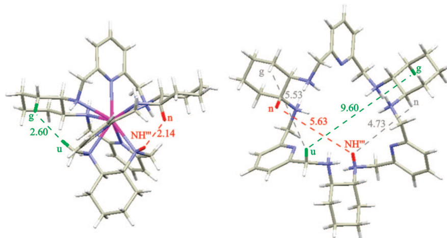
Figure 6. Comparison of the interproton distances between the structures of ( P )-[LuL RRRRRR ] 3+ complex (left) and the protonated free macrocycle (right). The two indicated colored distances correspond to the same pairs of protons ug (green) and NH''n (red).
