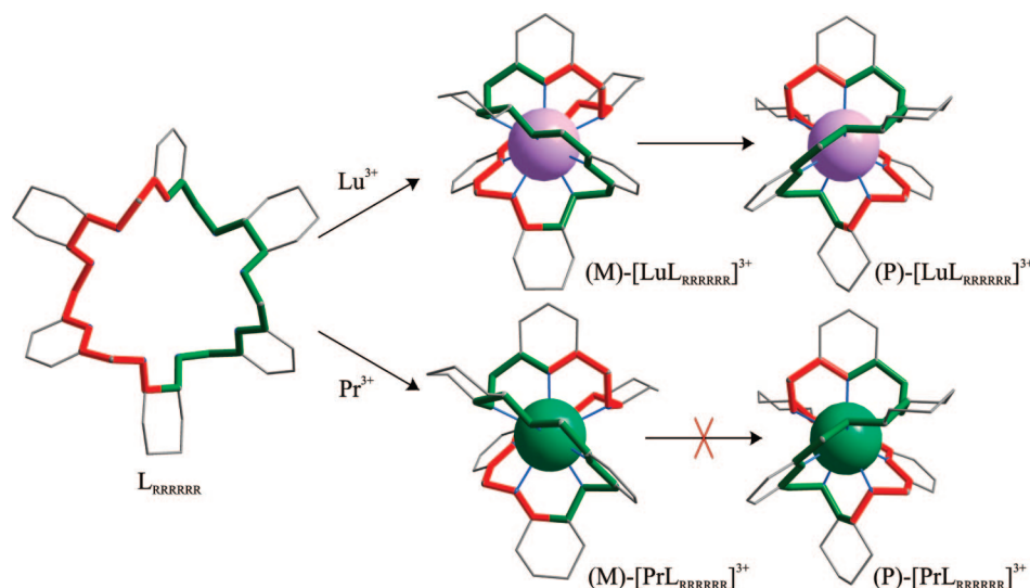
Scheme 2. Formation, Helicity Inversion and X-ray Crystal Structures a of the [LnL] 3+ Complexes
