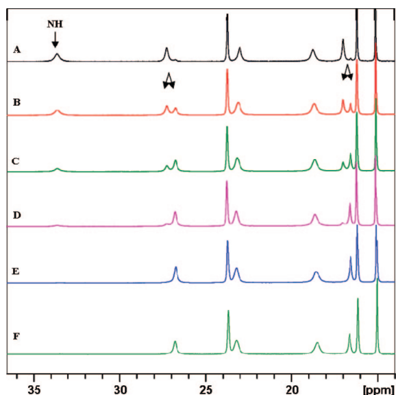
Figure 9. The fragments of the 1 H NMR spectra (298 K, \text{CD}_3\text{OD} ) of ( P )-[YbL RRRRRR ](NO 3 ) 3 ·6H 2 O complex, illustrating the disappearing of NH signal, doubling of the resonances due to isotope effect and the influence of added base. Traces A–E: spectra measured after 0.45, 1.45, 2.45, 4.45, and 27 h, respectively; trace F: spectrum of a sample containing 5 \mu\text{L} of \text{N}(\text{C}_2\text{H}_5)_3 measured after 0.25 h.
