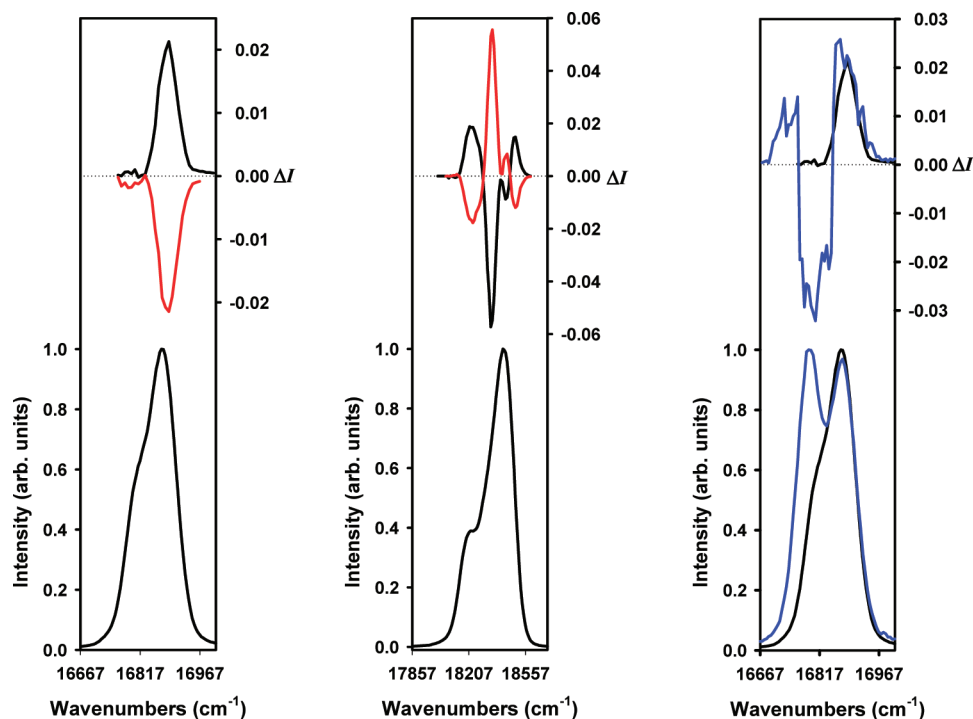
Figure 11. Circularly polarized luminescence (upper curve) and total luminescence (lower curve) spectra of ( M )-[LnL RRRRRR ] 3+ (Ln = Eu, Tb, black) and ( P )-[LnL SSSSSS ] 3+ (Ln = Eu, Tb, red) in 1 \times 10^{-2} M MeOH at 295 K, upon excitation at 283–284 nm, respectively. (Left) 5 D 0 → 7 F 1 (Eu) transition. (Middle) 5 D 4 → 7 F 5 (Tb) transition. (Right) 5 D 0 → 7 F 1 transition of ( M )-[EuL RRRRRR ] 3+ (black) and a 3.5:1 ( M )-[EuL RRRRRR ] 3+ :( P )-[EuL RRRRRR ] 3+ complex solution (blue).
