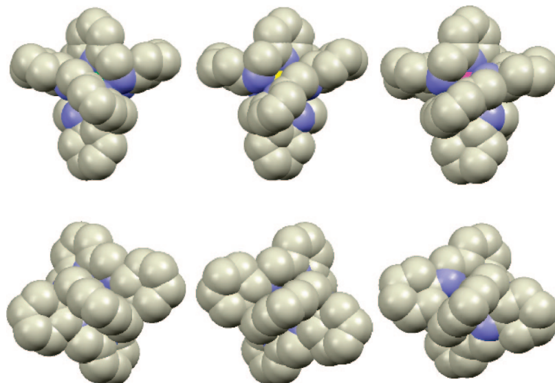
Figure 1. (Top) Views along the direction perpendicular to the C_2 axis of the structures of the (M) -[PrL RRRRRR ] 3+ (right), (P) -[CeL SSSSSS ] 3+ (middle) and (P) -[LuL RRRRRR ] 3+ (left) macrocyclic complexes. (Bottom) Views along the C_2 axis of the same complexes.
